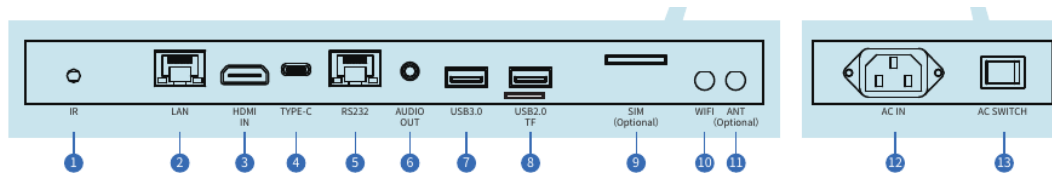
Figure 3 Connector layout
